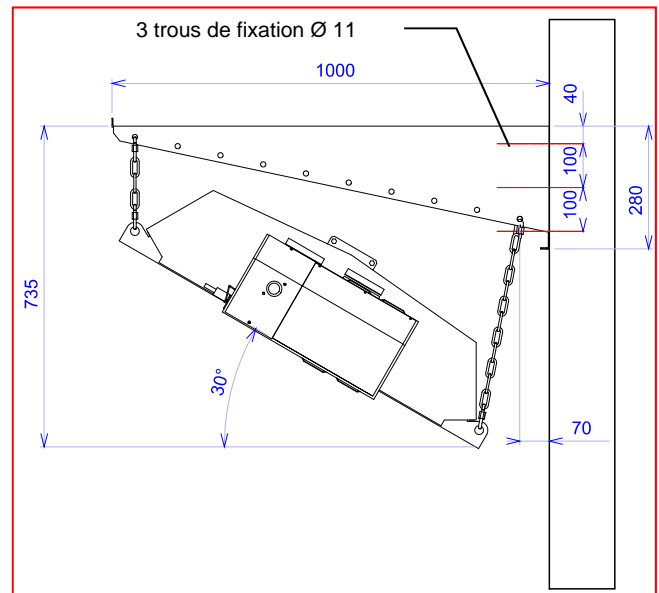
SUPPORT MURAL
