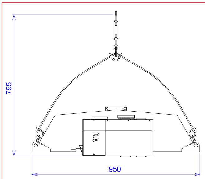
SUPPORT HORIZONTAL
